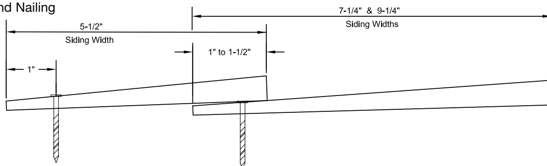
Figure 1: Blind Nailing
